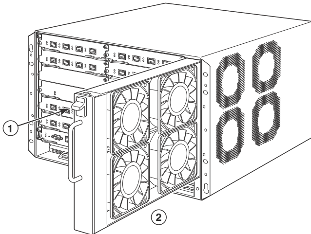
FIGURE 2 BigIron RX-8 Fan Assembly
