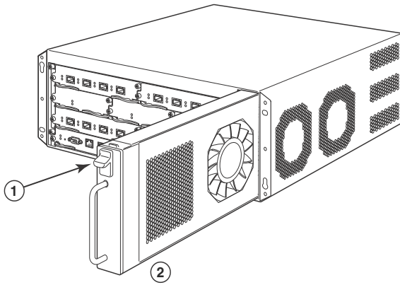
FIGURE 1 BigIron RX-4 Fan Assembly
